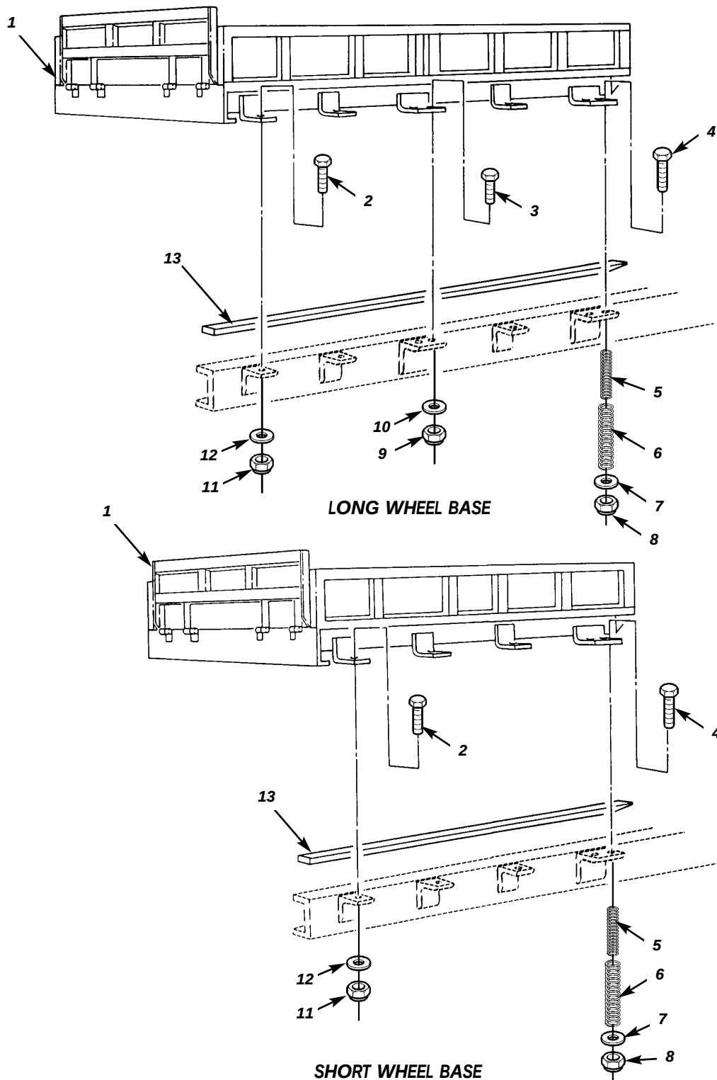
Figure 139. Cargo Body and Sill
