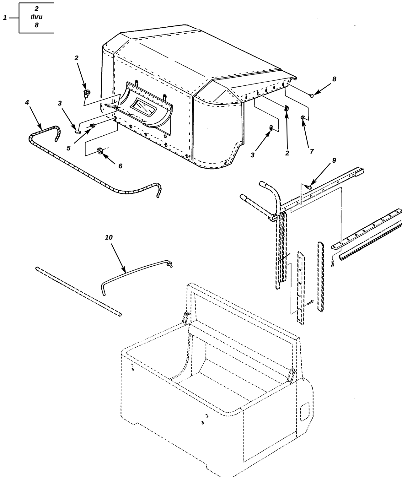
Figure 150. Cab Soft Top.
