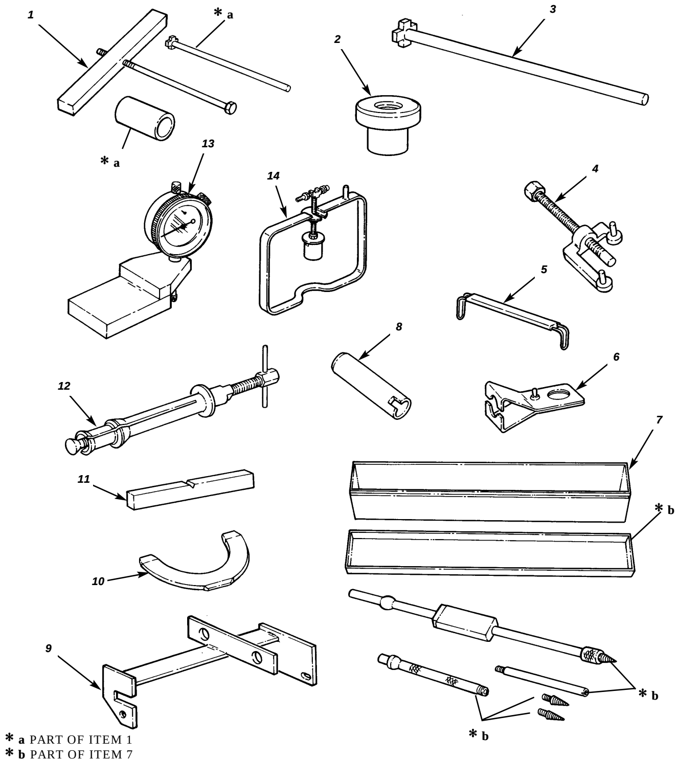
Figure 179 Special Tools (Sheet 1 of 2).
