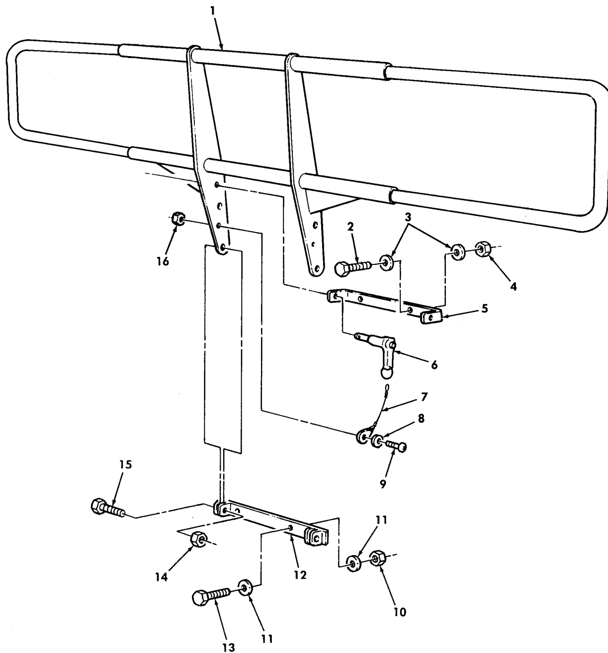
Figure 462. Brushguard Kit.
