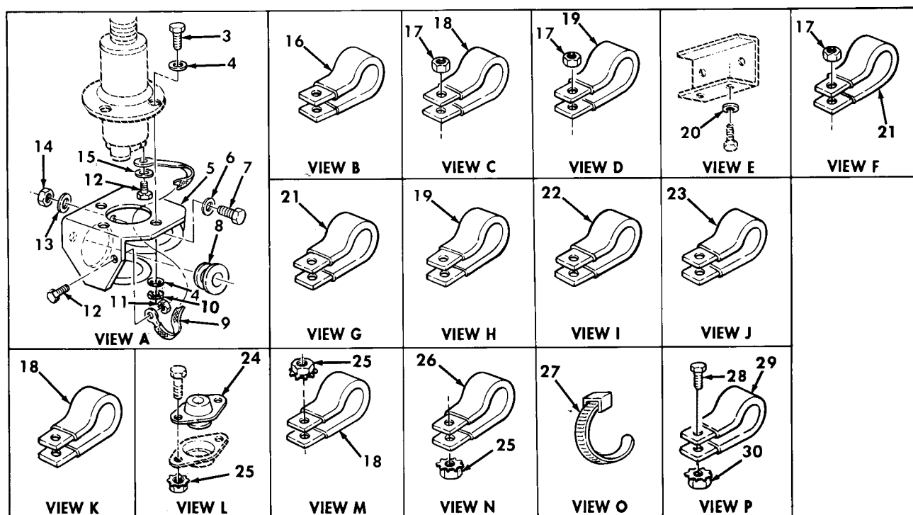
Figure 416. Communications Kit, Radio Cables, AN/VRC-49 and (2) TSEC/KY-57 Assemblies.
