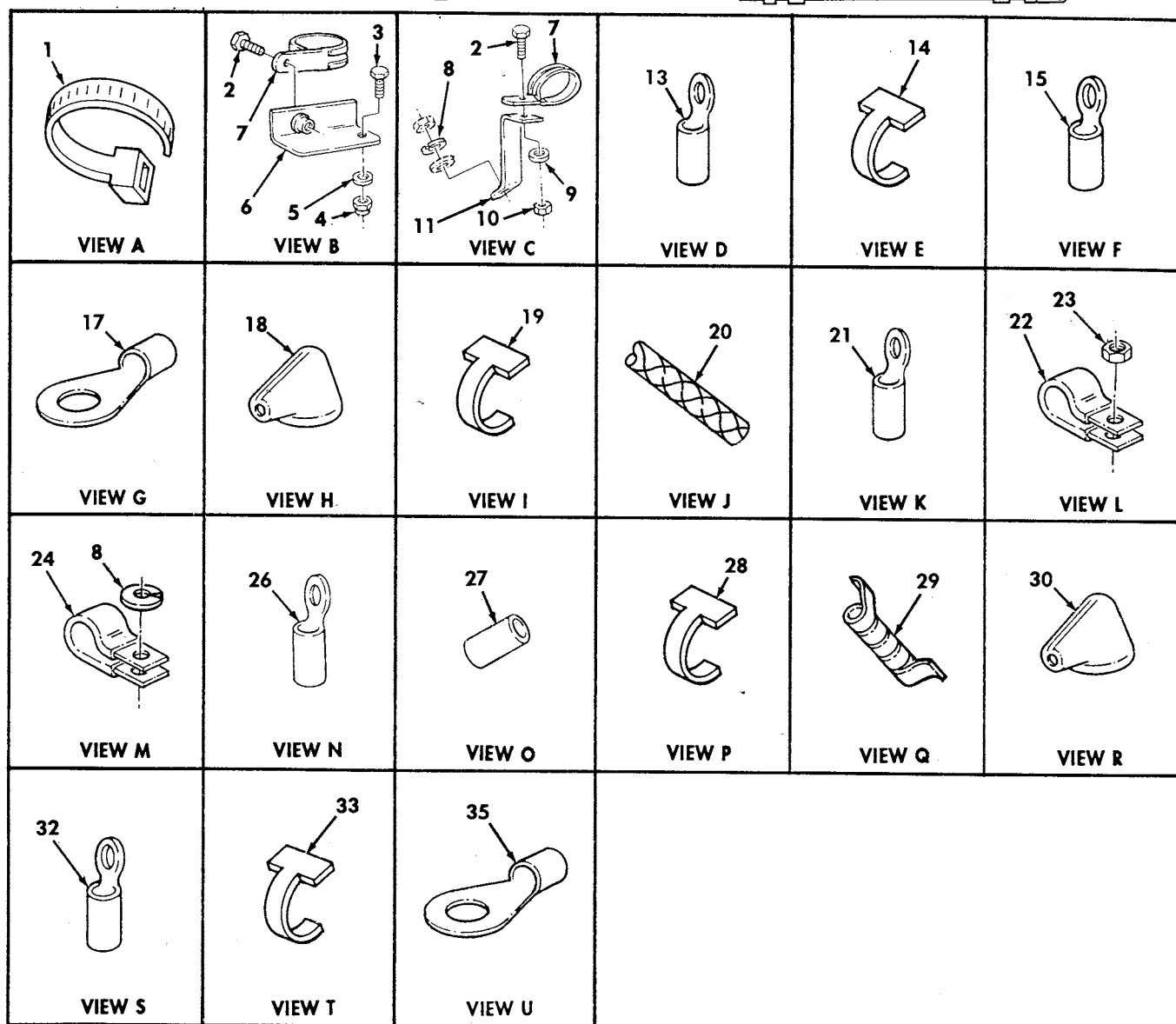
Figure 480. 400 AMP Alternator Wiring Harness Cable Assemblies.
